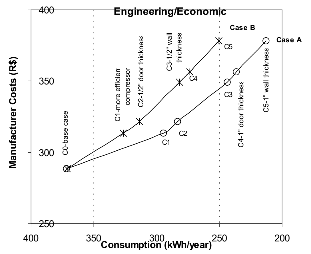
Figure 3: Engineering/Economic calculations
